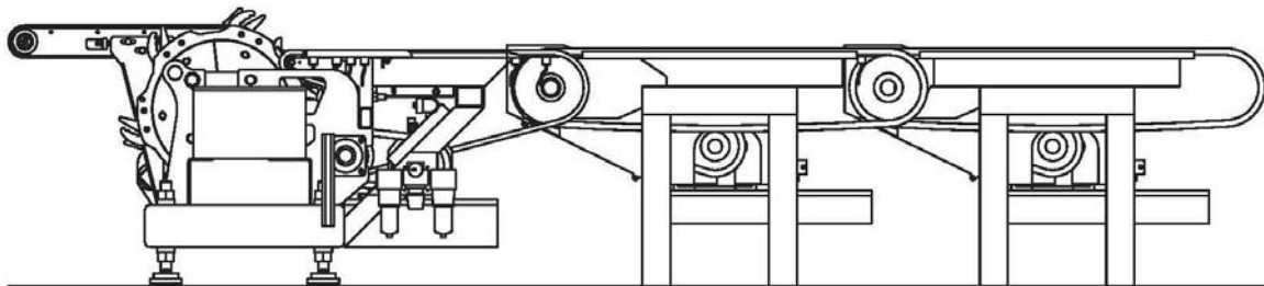
Pneumatic Rotor is used for all grabbing fingers and stoppers
