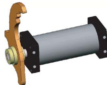
Pneumatic Rotor is used for all grabbing fingers and stoppers
